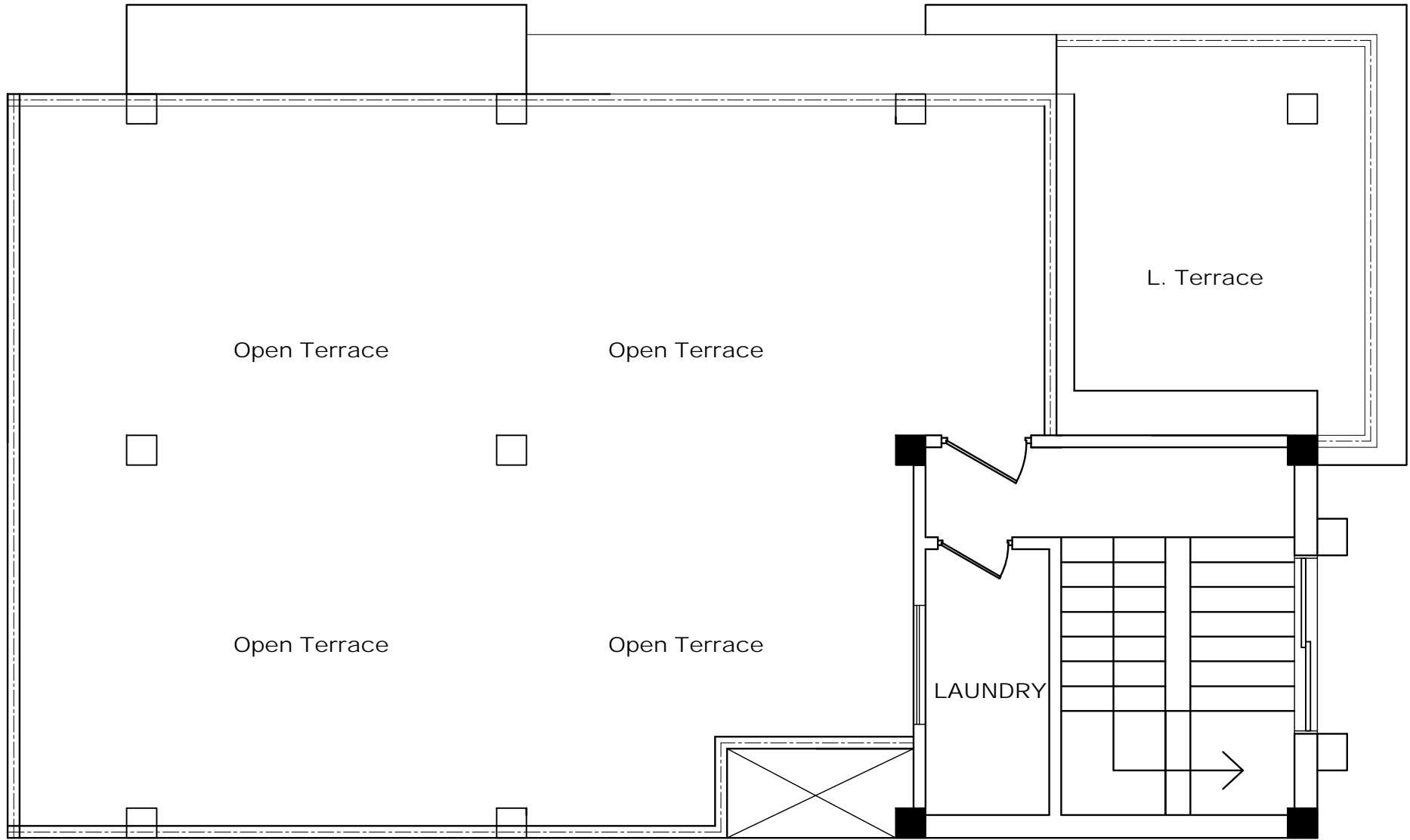
TOP FLOOR PLAN AREA: 17.25 SQ.M. (185.61 SQ.F.) all dimension are in cm
