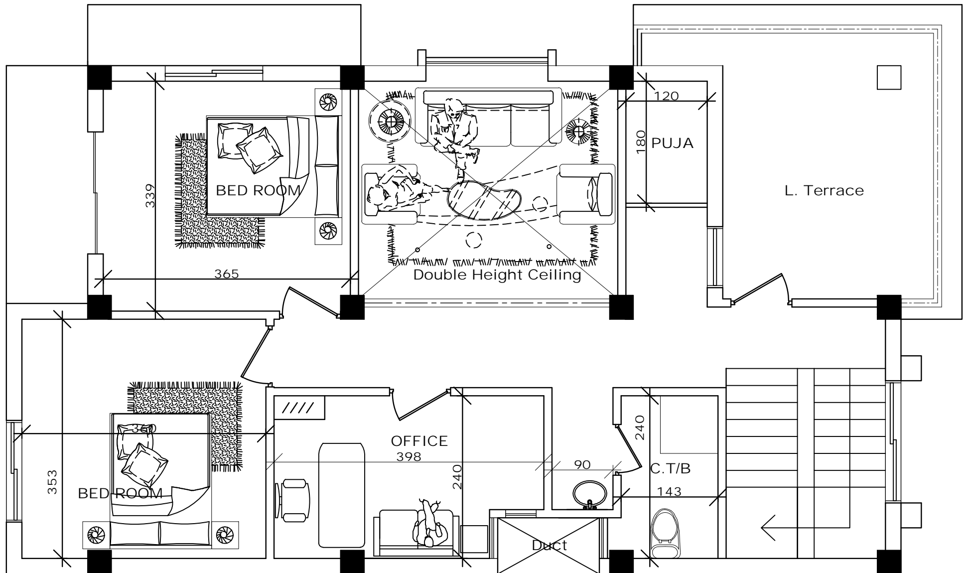
SECOND FLOOR PLAN AREA: 85.74 SQ.M. (922.56 SQ.F.) all dimension are in cm
