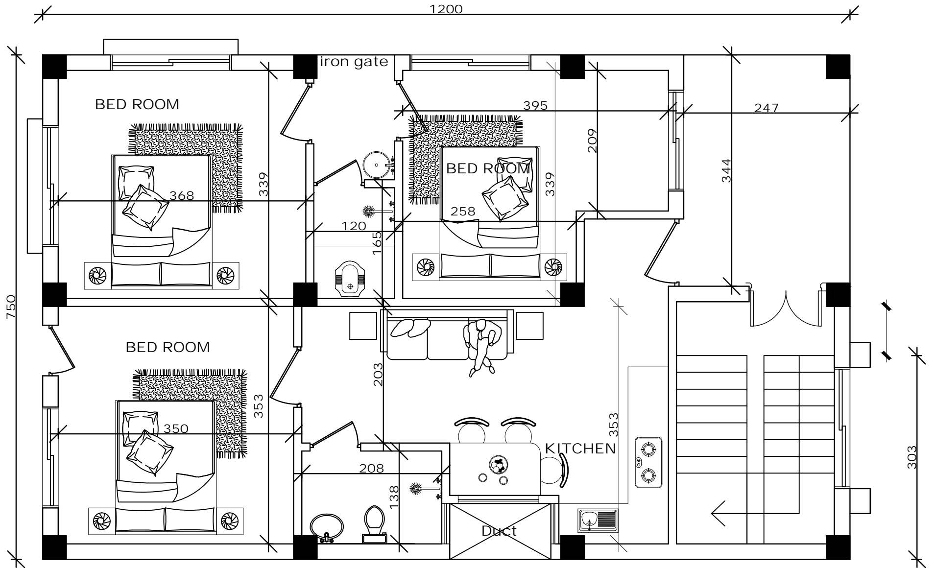
GROUND FLOOR PLAN AREA: 90.00 SQ.M. (968.40 SQ.F.) all dimension are in cm
